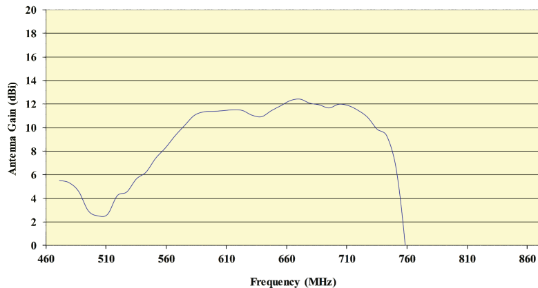
Antenna Gain (dBi) vs. Frequency (MHz)
